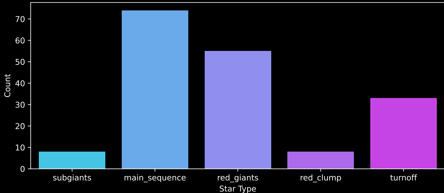
APOGEE DR17 Field: [INTCL_N5634_MGA] Count plot of Star Type
