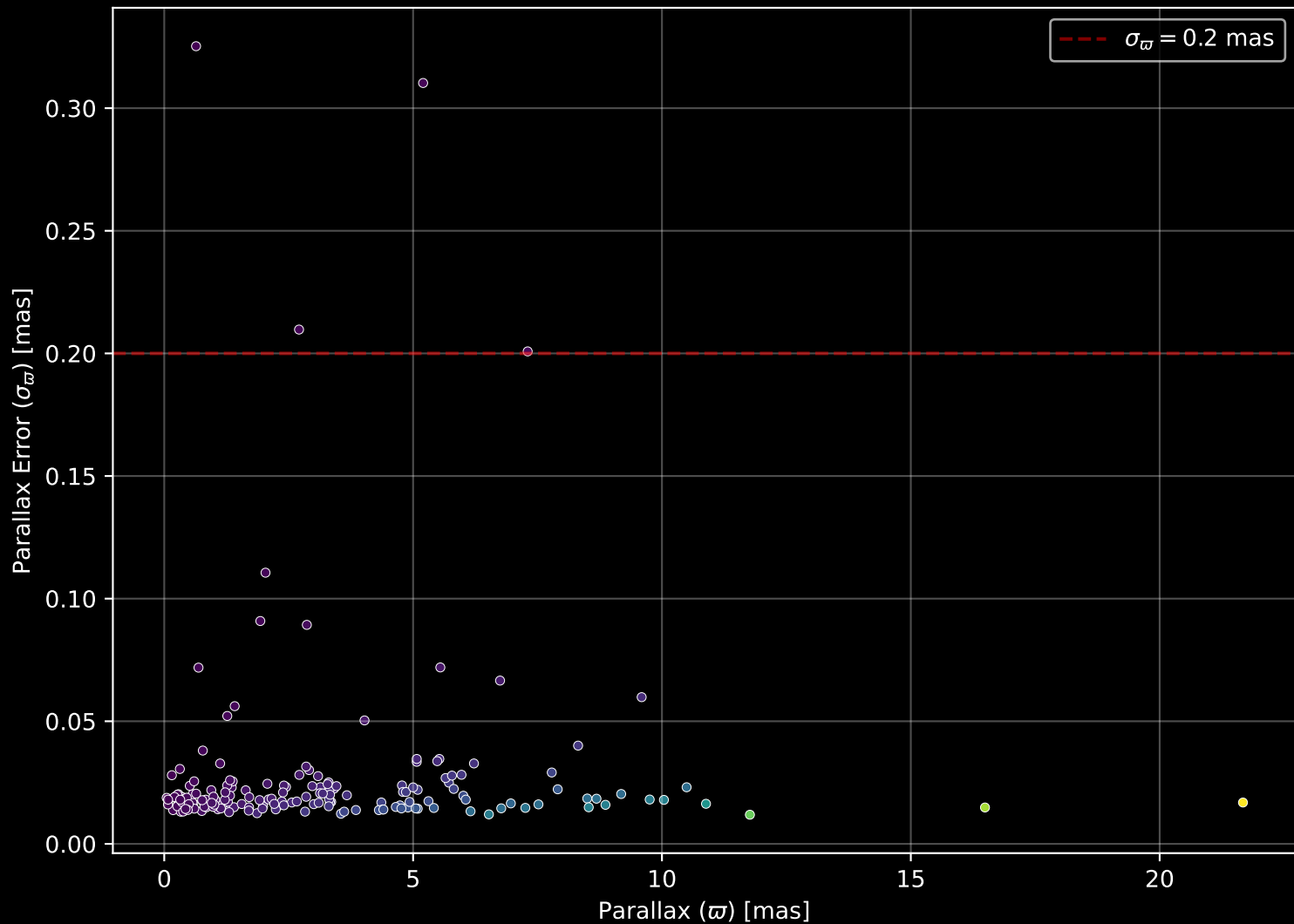
APOGEE DR17 Field: [INTCL_N5634_MGA] Parallax Quality (n= 178)
