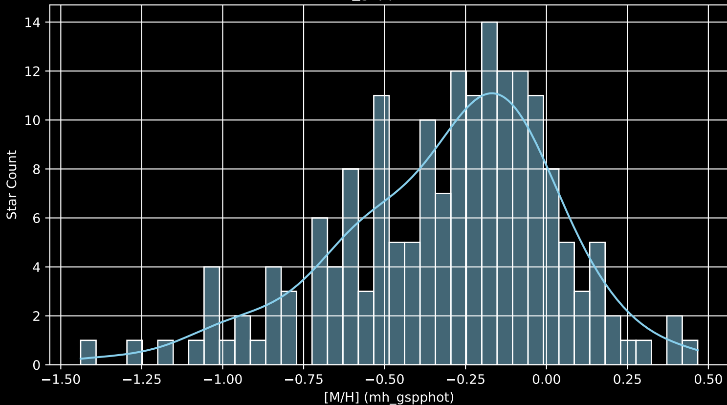
APOGEE DR17 Field: [INTCL_N5634_MGA [M/H] (mh_gspphot) (n= 178)
