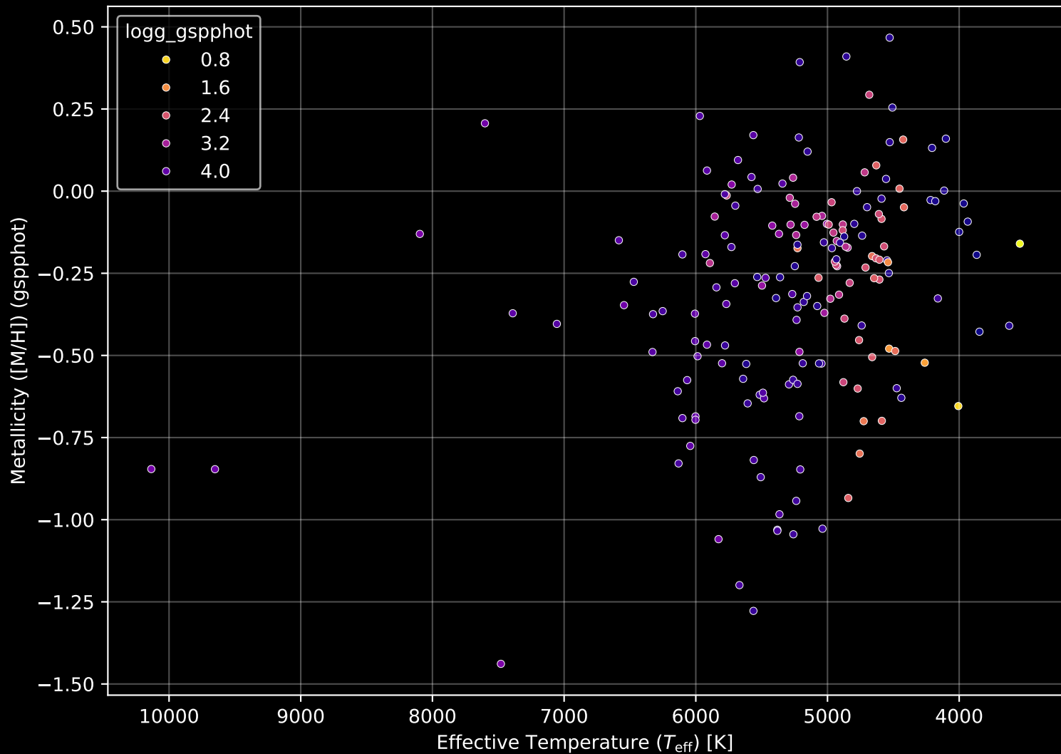
APOGEE DR17 Field: [INTCL_N5634_MGA] Stellar Population Parameters (n= 178)
