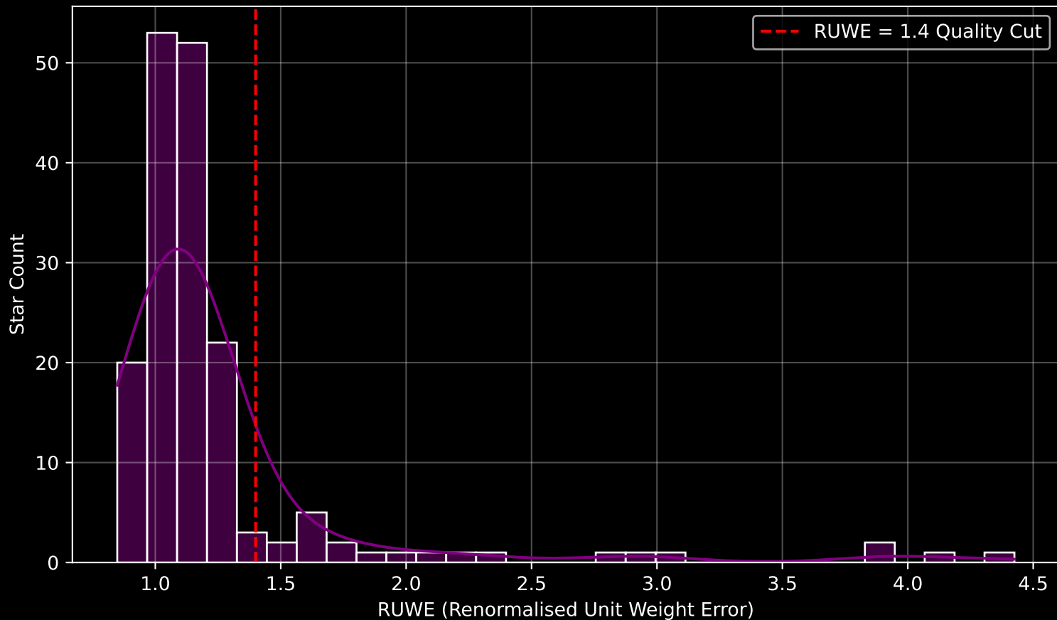
GAPOGEE DR17 Field [INTCL_N5634_MGA] RUWE Distribution (n= 171)
