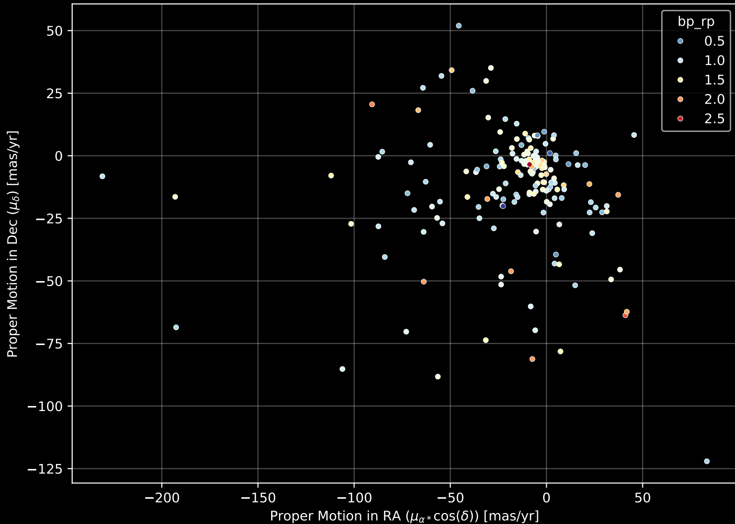
APOGEE DR17 Field: [INTCL_N5634_MGA] Proper Motion Diagram (n= 178)
